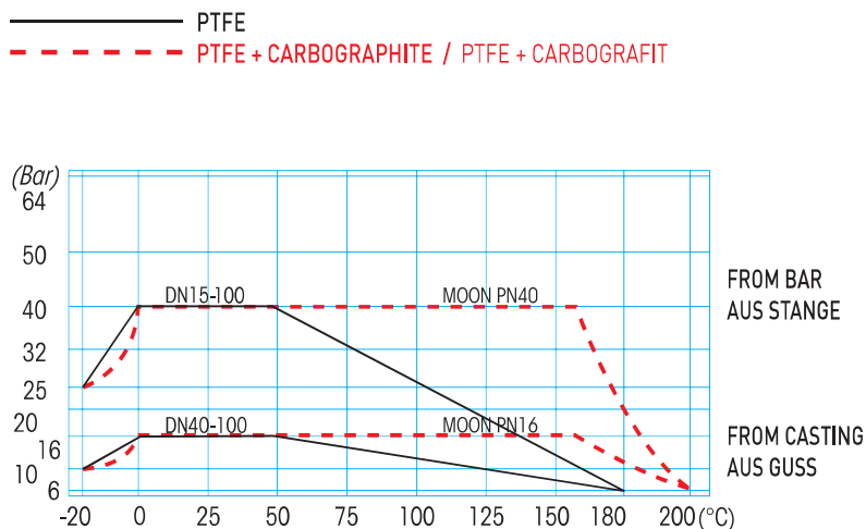
PRESSURE/TEMPERATURE DIAGRAM / DRUCK- / TEMPERATURDIAGRAMM
